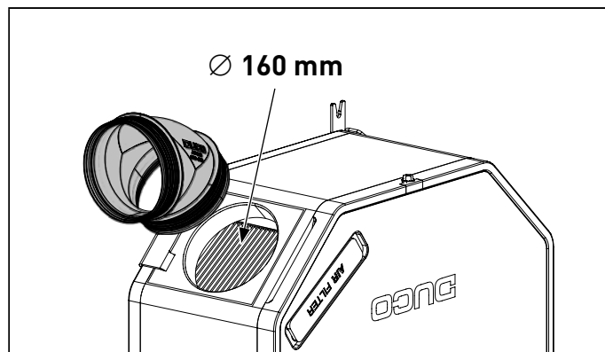
Slide the connection piece into the unit
