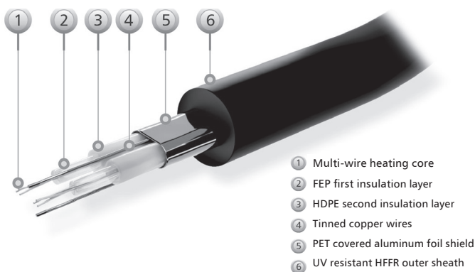
ELEKTRA SnowTec ® Tuff heating mat's cable structure
