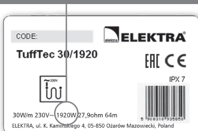
Self-adhesive label
