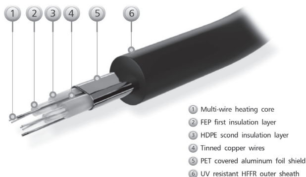
Construction of the ELEKTRA TuffTec™ heating cable
